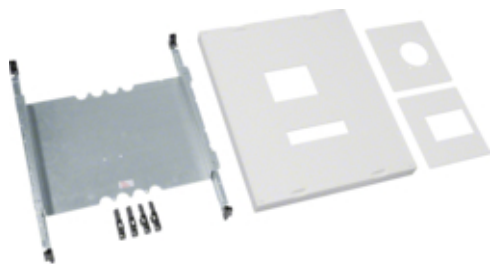
univers N Blok do MCCB 400/630A +RCD
